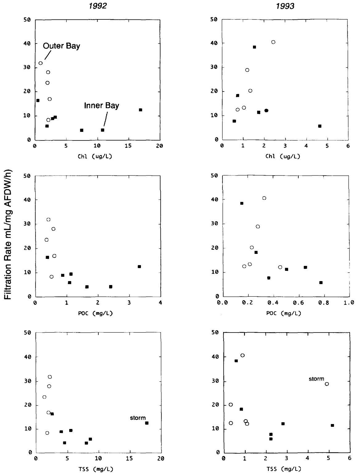
FIG. 3. Relationship between filtration rate and seston concentration for Dreissena polymorpha on each sampling date in 1992 and 1993 at a site in the inner bay and outer bay of Saginaw Bay. chl = chlorophyll ; POC = particulate organic carbon; TSS = total suspended solids.
