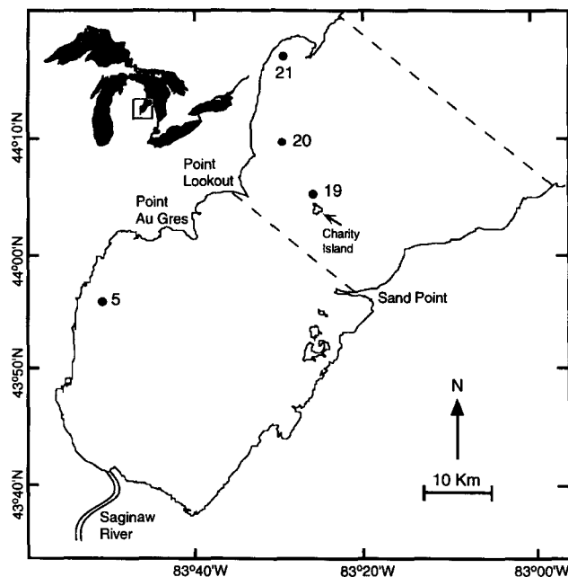
FIG. 1. Location of sampling sites in Saginaw Bay, Lake Huron. Dashed lines differentiate the inner bay from the outer bay and the outer bay from Lake Huron.
