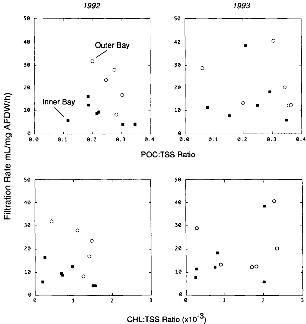
FIG. 4. Relationship between filtration rate and seston composition for Dreissena polymorpha on sampling date in 1992 and 1993 at a site in the inner bay and outer bay of Saginaw Bay. Seston composition is defined as the proportion of particulate organic carbon in the total material suspended (POC:TSS) and as the proportion of chlorophyll in the total material suspended (chl:TSS).
