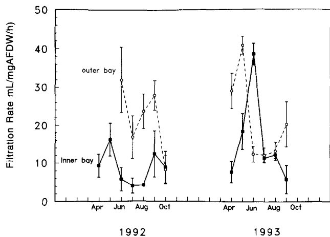
FIG. 2. Mean ( \pm SE) filtration rates for Dreissena polymorpha on each sampling date in 1992 and 1993 on seston from a site in the inner bay and a site in the outer bay of Saginaw Bay.
