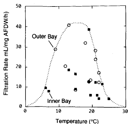
FIG. 5. Relationship between filtration rate and temperature for Dreissena polymorpha on each sampling date in 1992 and 1993 at a site in the inner bay and outer bay of Saginaw Bay. The dashed line is fitted to maximum filtration rates over the range of seasonal temperatures.
